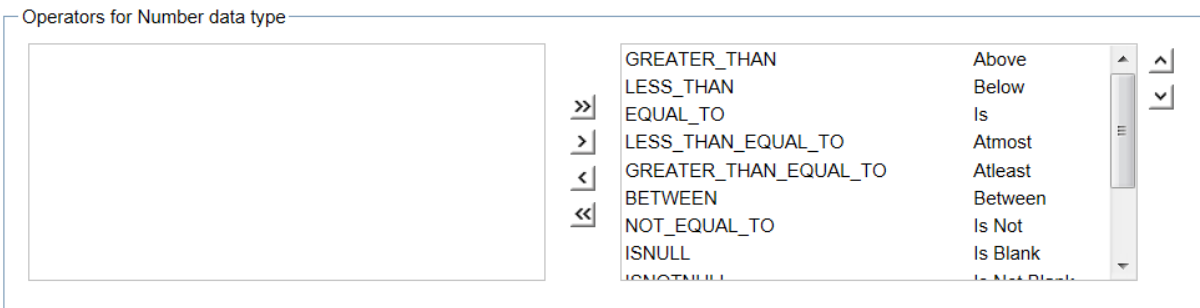
Figure 10: Filter Operators for number data type
