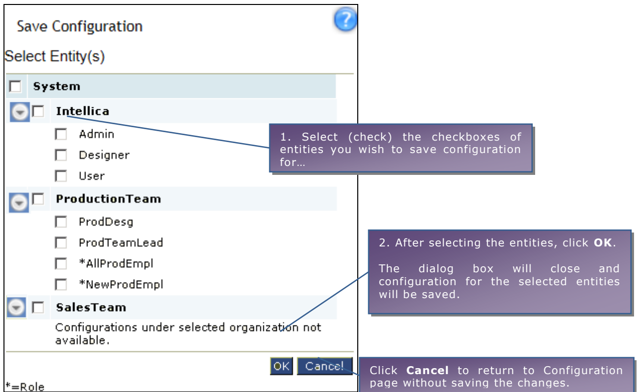
Figure 3: Save Configuration dialog
