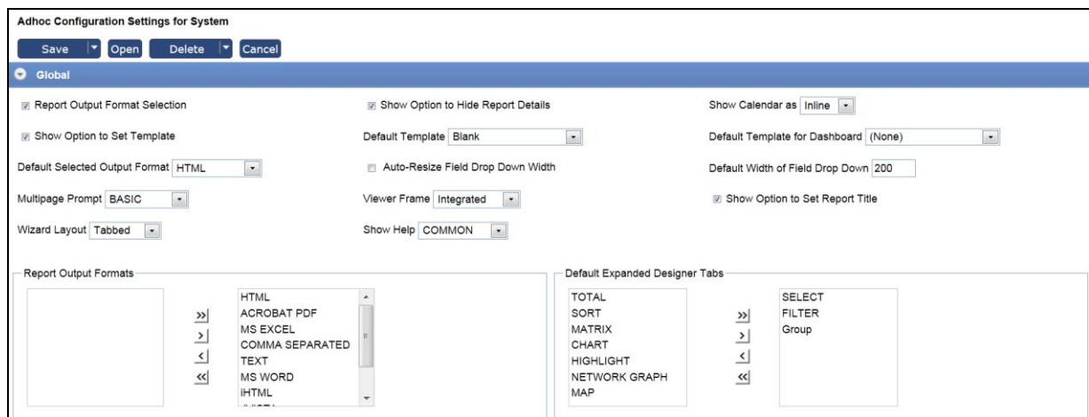
Figure 5: Configuration page for Adhoc Wizard
