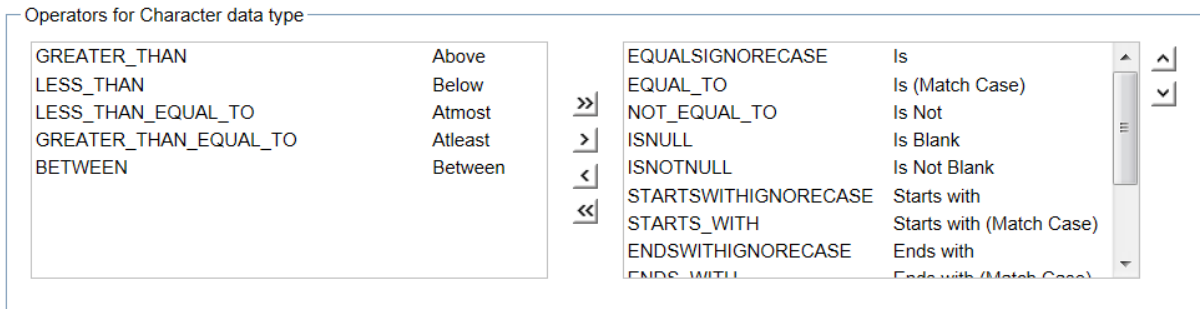
Figure 9: Operators for Character data type
