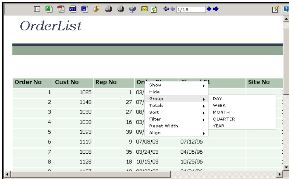
Figure 11: Grouping by Date Field
