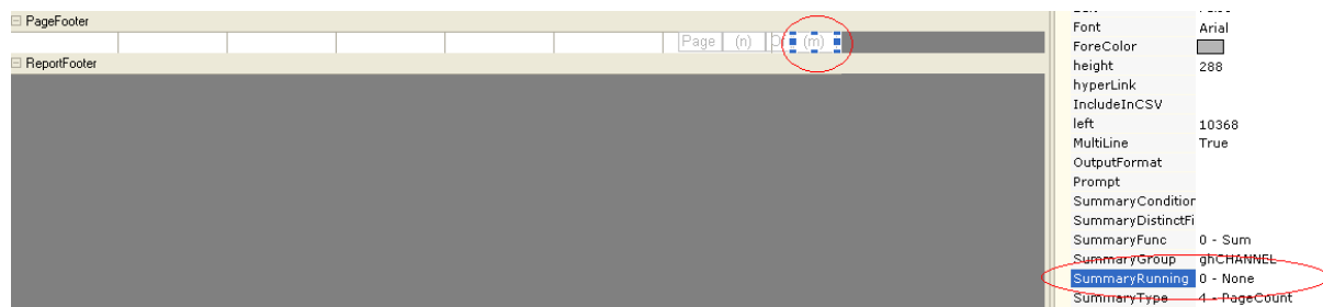
Figure 39: Summary Group
