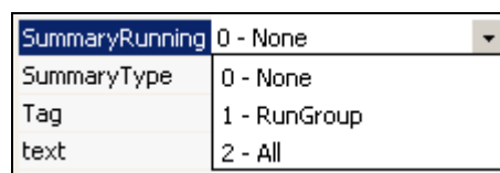
Figure 40: Summary Running
