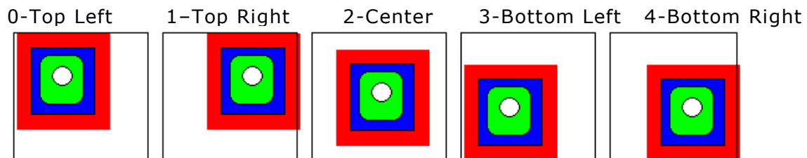
Figure 35: Picture Alignment
