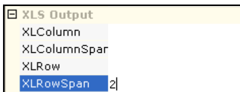
Figure 50: XLRowSpan
