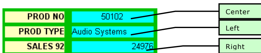
Figure 4: Alignment
