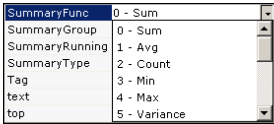
Figure 38: Summary Function
