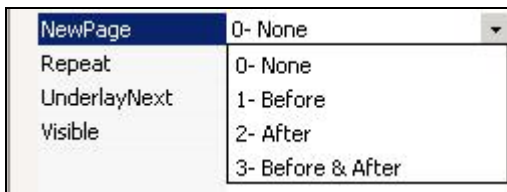
Figure 34: New Page
