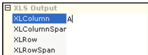
Figure 46: XL Column
