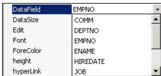
Figure 19: Data Fields
