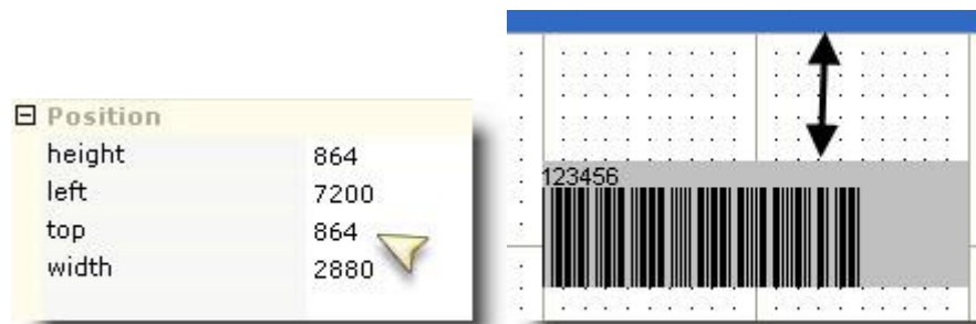
Figure 42: 'Top' Property
