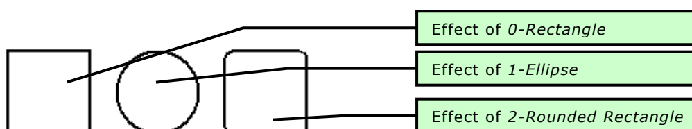
Figure 36: Shapes
