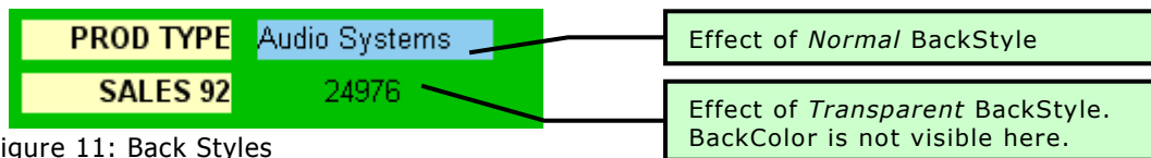
Figure 11: Back Styles
