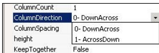
Figure 17: Column Direction
