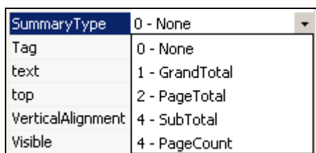
Figure 41: Summary Types
