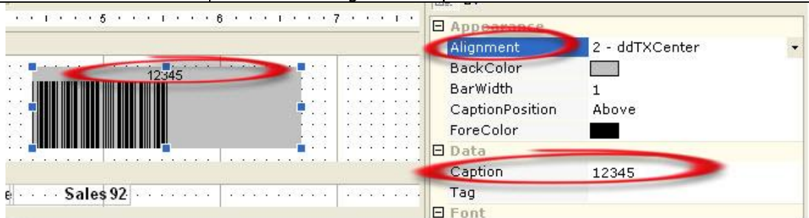
Figure 5: Alignment
