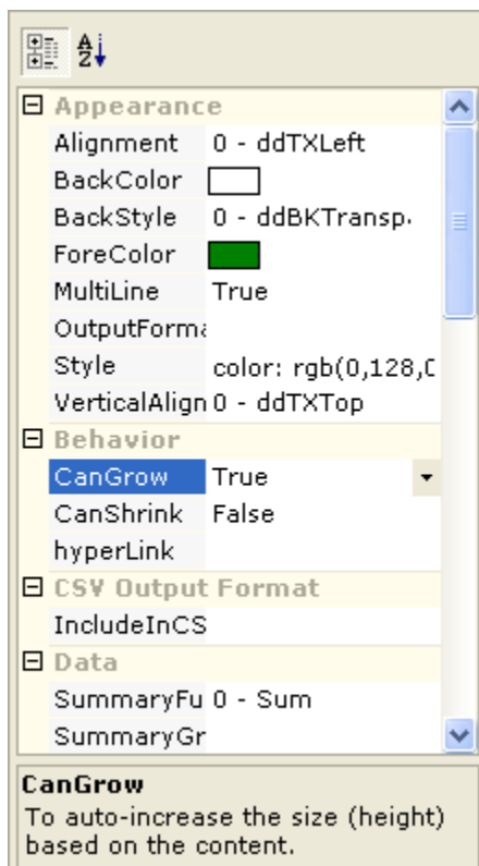
Figure 1: Properties List
