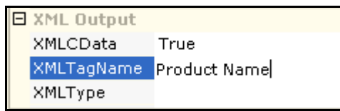
Figure 52: XMLTagName
