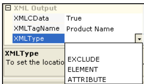
Figure 53: XMLType
