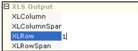
Figure 49: XLRow
