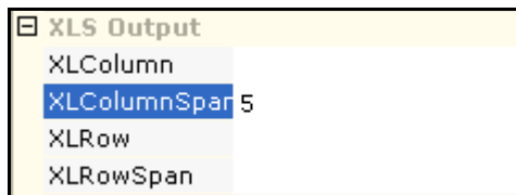
Figure 47: XLColumnSpan
