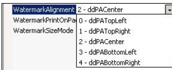
Figure 45: Watermark Alignment
