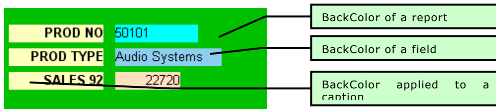
Figure 6: Back Color
