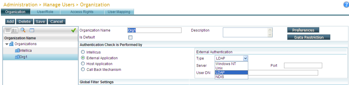
Figure 3: External Application-LDAP
