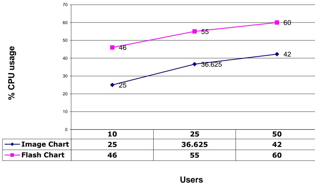
Maximum CPU usage - (Flash Chart v/s Image Chart)
