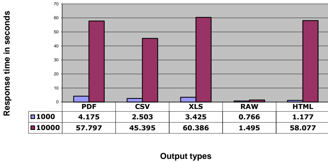
Report execution time - (Records v/s output types)
