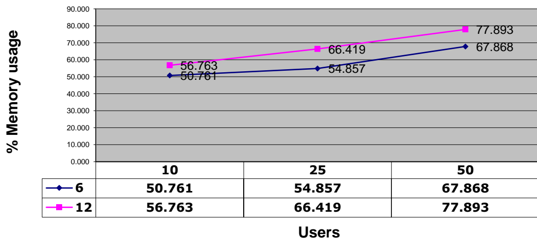
Maximum Memory Usage (SMART Report of different chart types)
