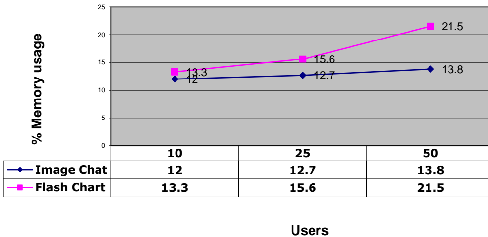
Maximum Memory usage - Flash Chart v/s Image Chart)
