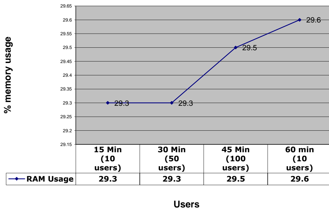
RAM usage - Resource usage trend
