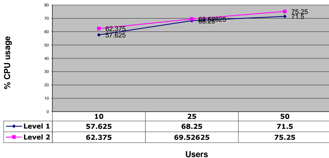
Maximum CPU usage - Sub-report levels v/s users
