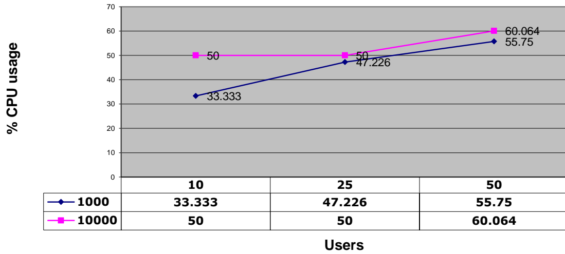
Maximum CPU Usage (SMART Report)
