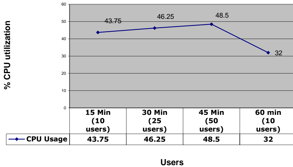
CPU Usage - Resource usage trend
